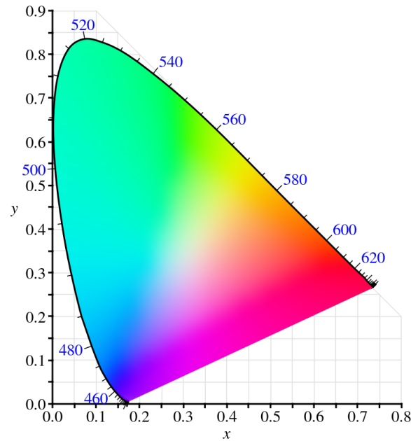
Figure 3: Chromaticity diagram
